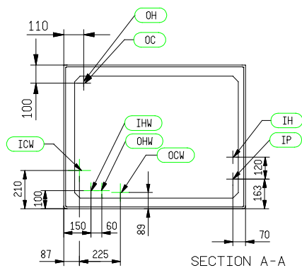
FRONTAL SUCTION VERSION
